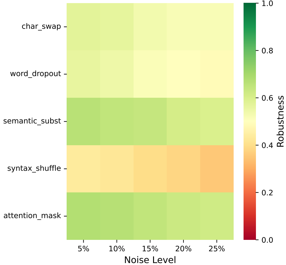
DistilBERT
