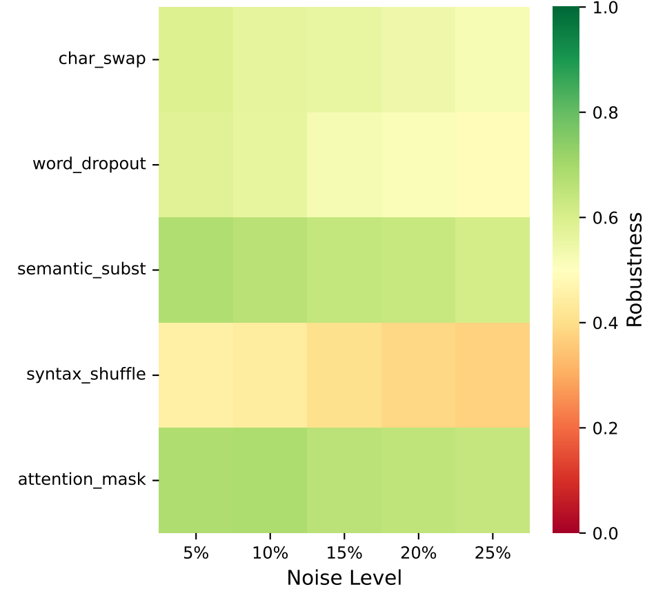
ALBERT-base
