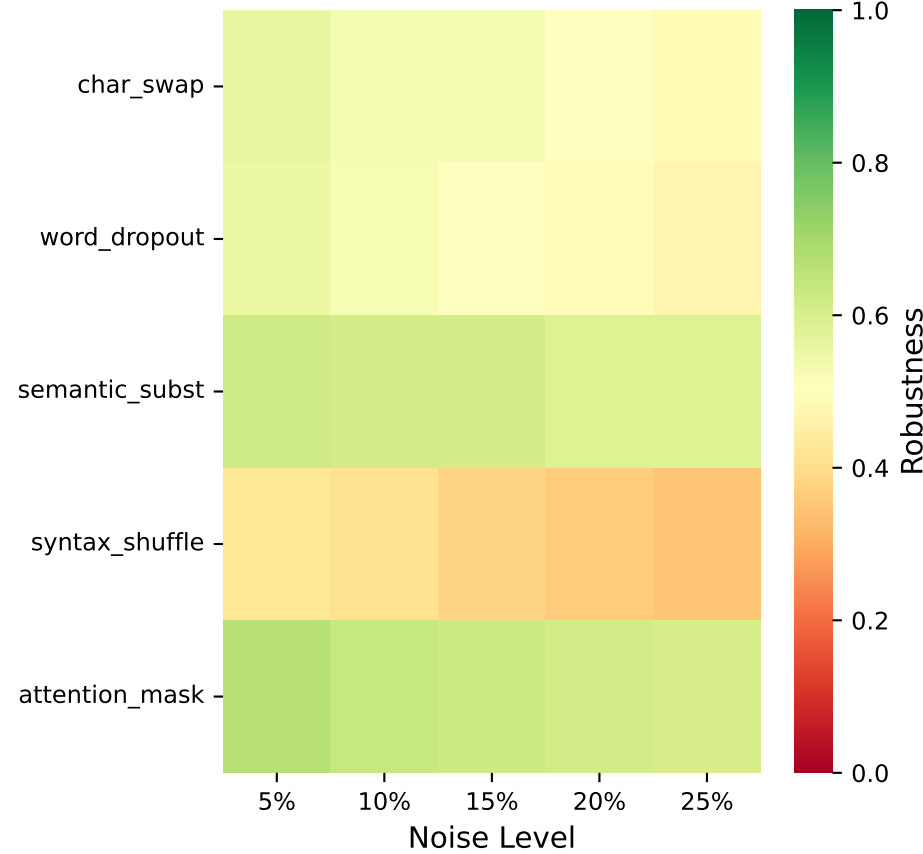
ELECTRA-small
